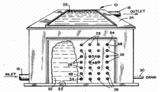
Figure 2. A semi-pressurized UV system where the UV lamps are perpendicular to the flow and the quartz sleeves are cleaned by circulating acid through the tank.
