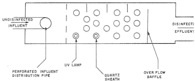
Figure 11. The UV system used by Ho and Bohm showing the baffles to prevent short circuiting along the top surface of the UV unit.
